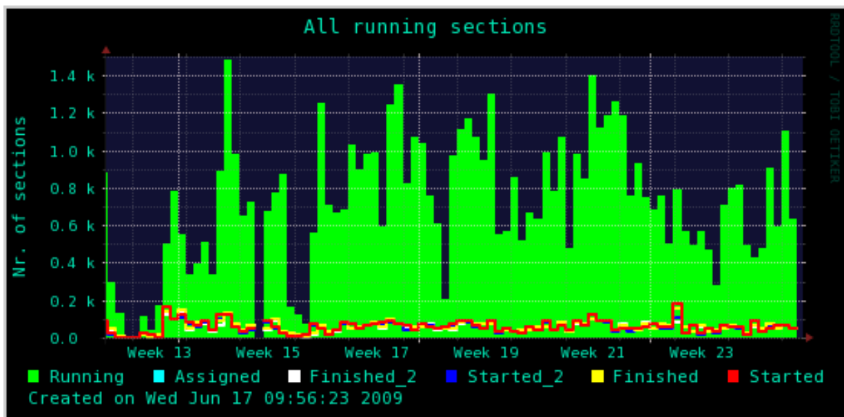
Figure 2: Running CDF jobs on NAMGrid
