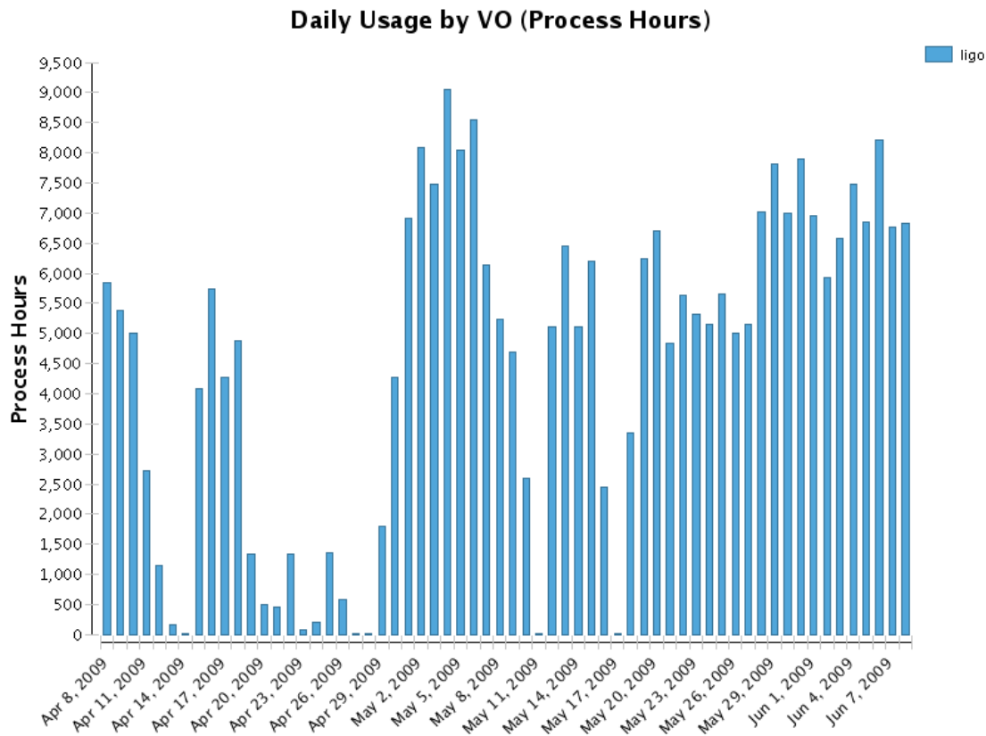
Figure 1: OSG Usage by LIGO's Einstein@Home application for the two month period covering both the month before full deployment of the new code and the first month of running at production levels with the new code using the GRAM 2 job submission interface.
