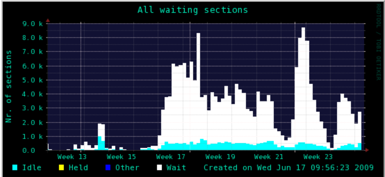
Figure 3: Waiting CDF jobs on NAMGrid
