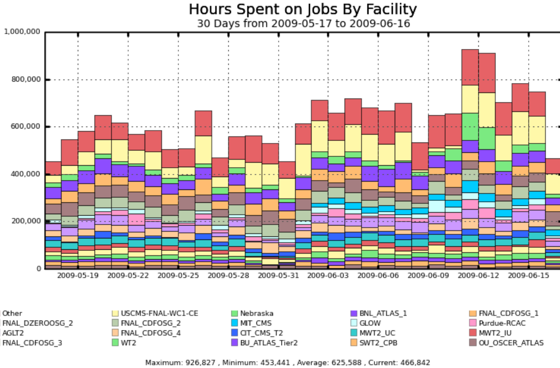
Figure 10: OSG facility usage vs. time broken down by Site. (Other represents the summation of all other “smaller” sites)
