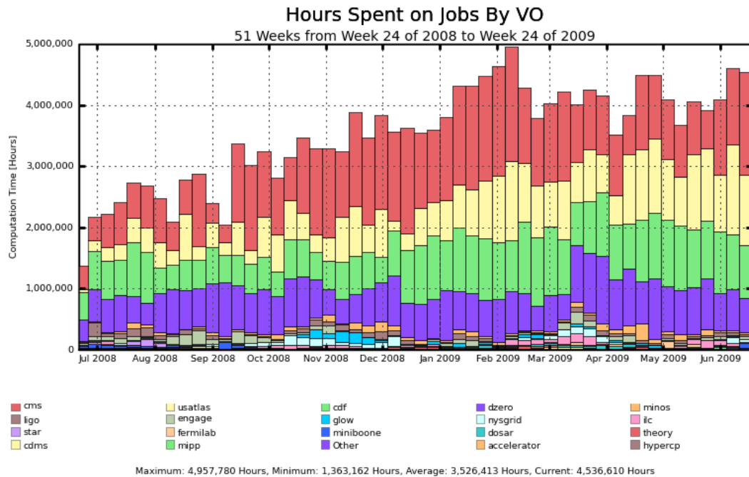
Figure 9: OSG facility usage vs. time broken down by VO
